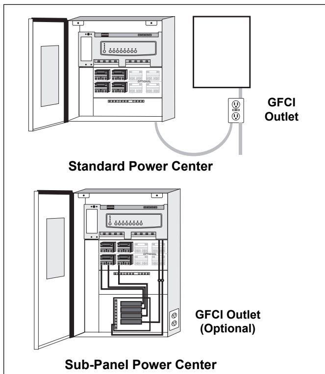
Figure 4. GFCI Installation for Underwater Lighting
